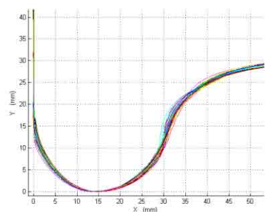
Comparative measurement of multiple profiles
