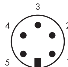
M16 Stecker M16 connector
