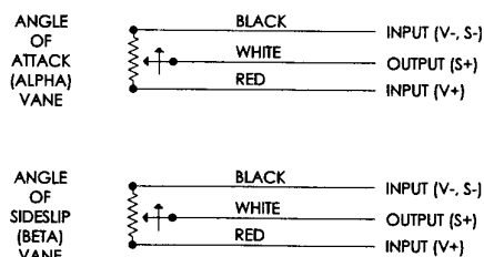
ELECTRICAL SCHEMATIC
