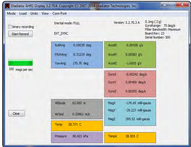
AHRS Data in Full Mode at 200Hz Data Rate
