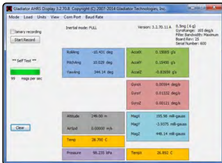
AHRS Selectable 100-200 Hz Data Rate
